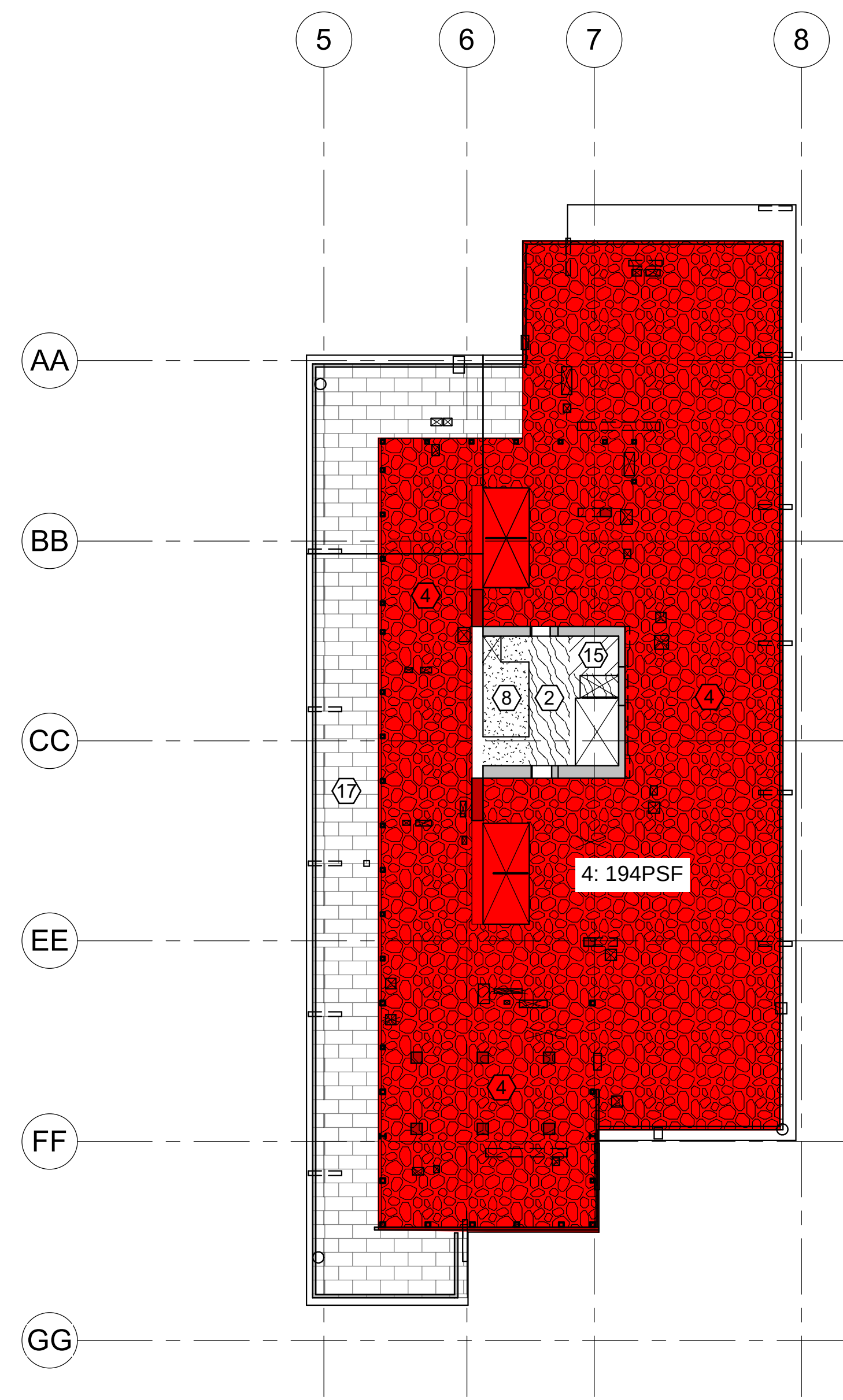
3 ROOF LOAD DIAGRAM SCALE: 1" = 20'-0"
