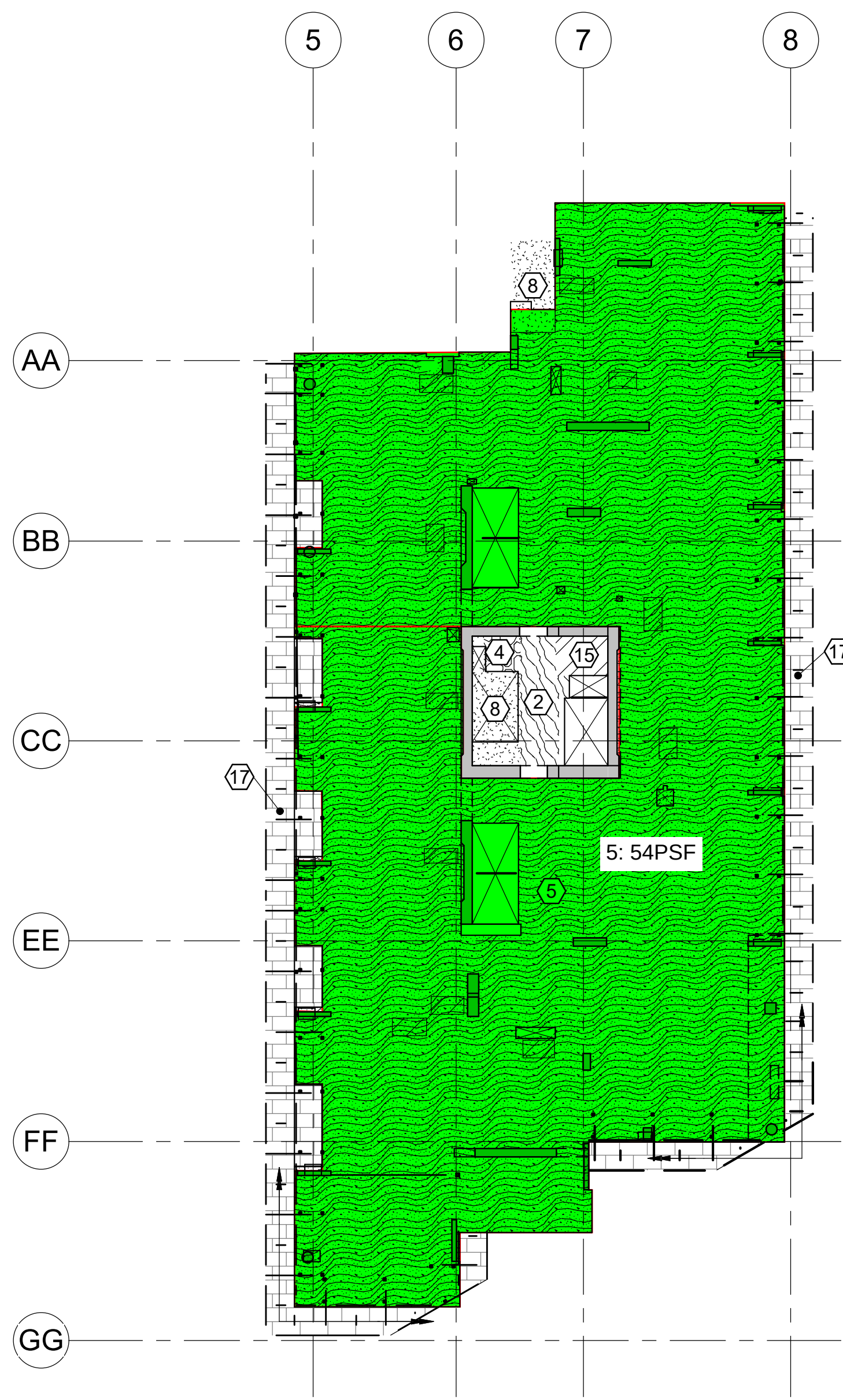
1 LEVEL 6 LOAD DIAGRAM SCALE: 1" = 20'-0"
