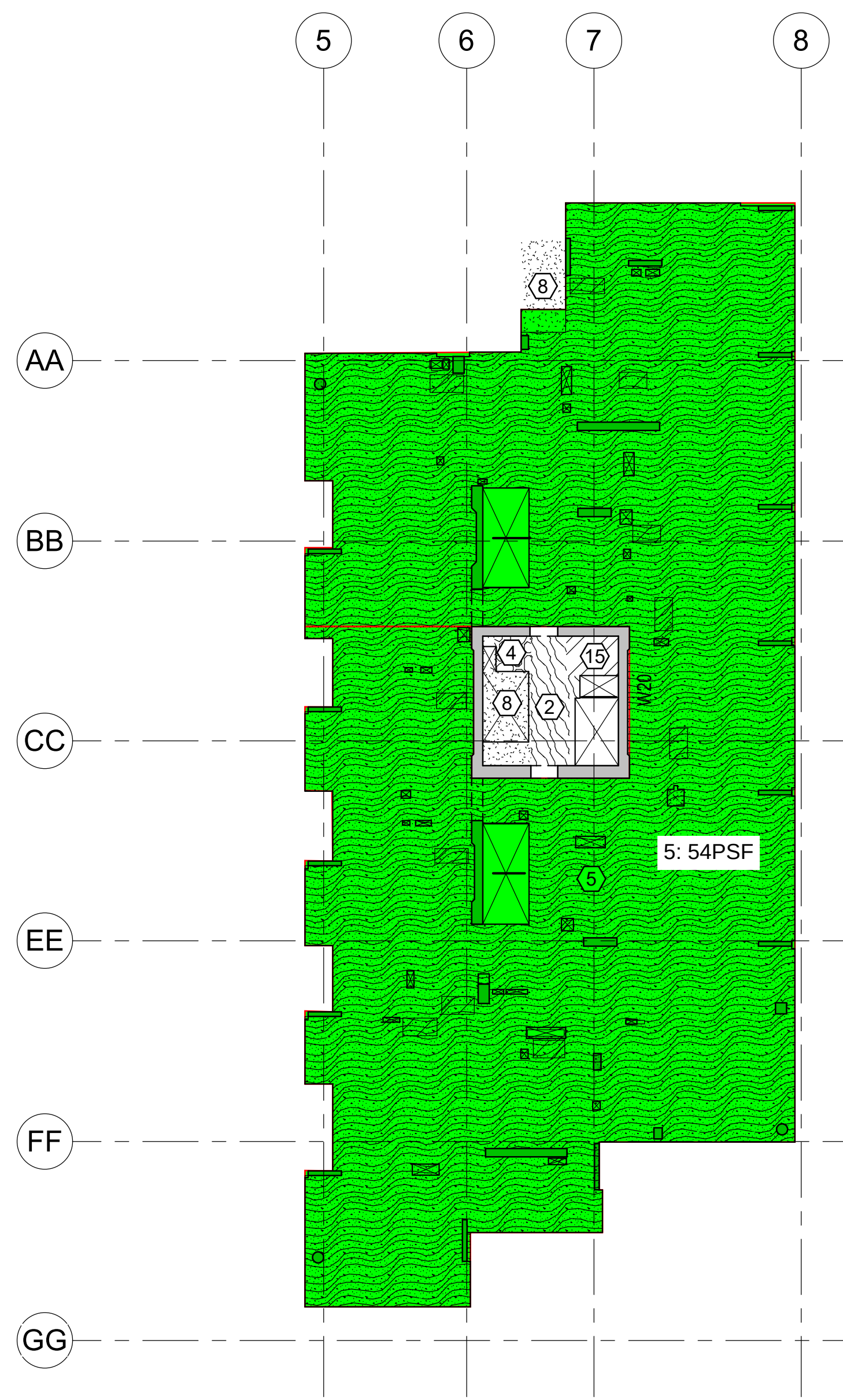
2 LEVEL 7-38 LOAD DIAGRAM SCALE: 1" = 20'-0"
